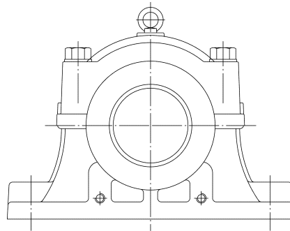
SDAF500/600/00K
